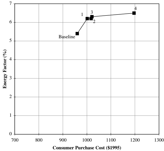
Figure 11.9. Cost Versus Efficiency for New Gas Ovens (Self-Cleaning)
