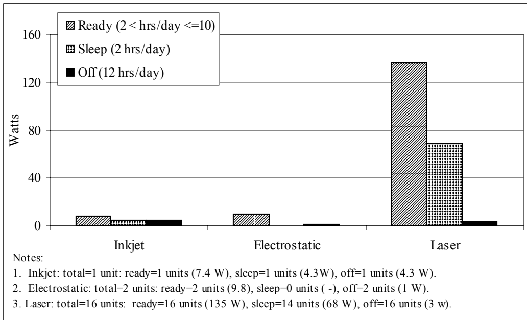
Figure 11: Results for Photocopiers by Copy Engine
