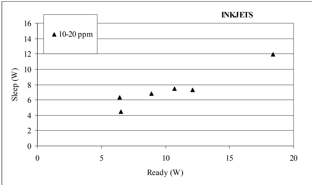
Figure 8: Distribution of Ready Power vs. Sleep Power by Print Engine
