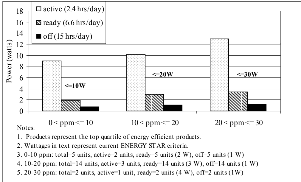
Figure 2: Results for Print-only Inkjets
