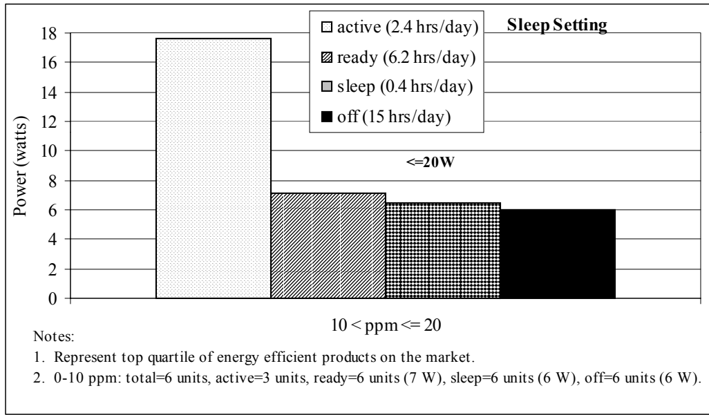
Figure 3: Results for Inkjet Printer-Based MFDs
