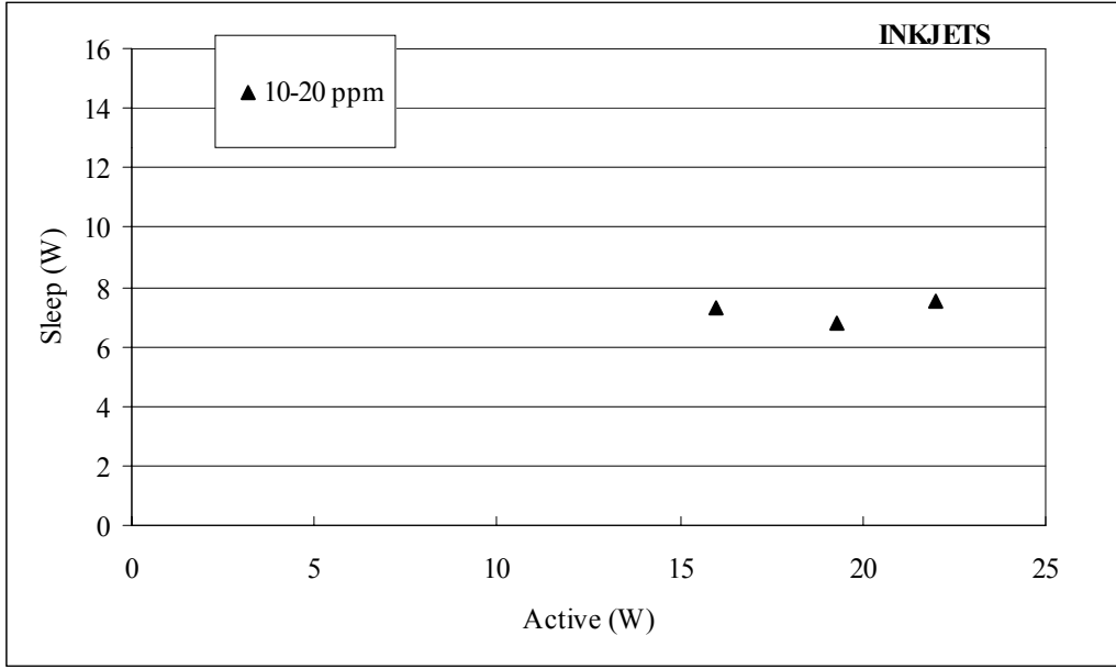
Figure 7: Distribution of Active Power vs. Sleep Power by Print Engine
